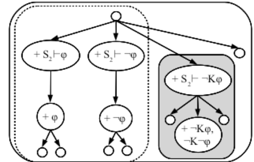
Figure 11: Answer I don't know .
