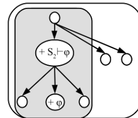
Figure 12: Monopolar question, ?{φ}
