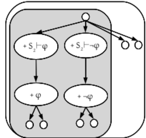
Figure 9: Polarity question ? \{\varphi, \neg\varphi\}
