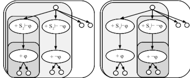
Figure 10: Answers yes / no
