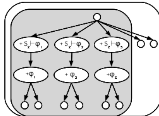
Figure 15: Asking a constituent question
