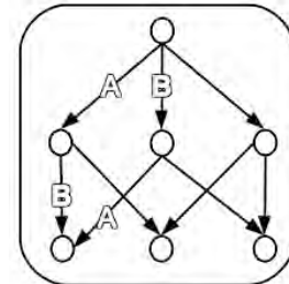
Figure 4: Reaching the same commitment state by different paths
