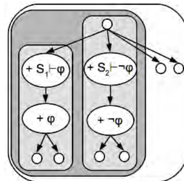
Figure 25: Disjunction of assertion and monopolar question of its negation: A proper CS
