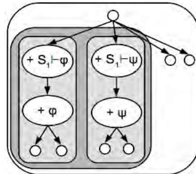
Figure 24: Disjunction of two assertions: Not a proper CS
