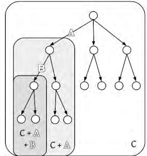
Figure 6: Commitment space development
