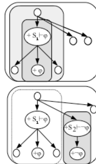
Figure 13: Answers yes / no to monopolar question
