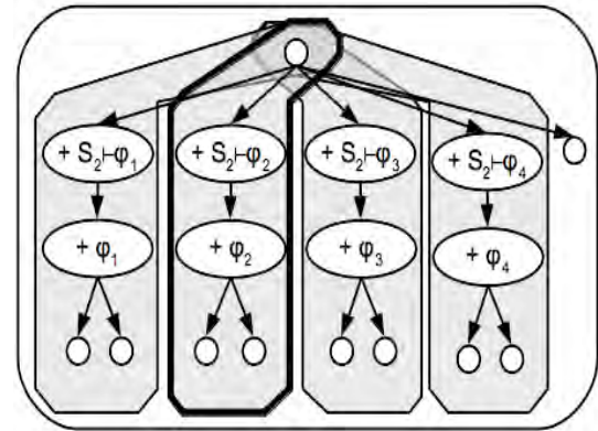
Figure 20: Alternatives of question Did JOHN arrive? , highlighted: Did John arrive?
