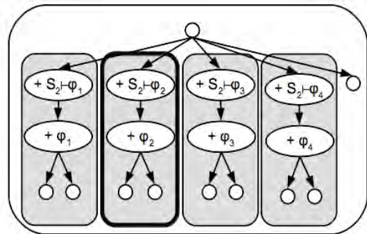
Figure 18: Alternatives of assertion JOHN arrived ; the assertion itself ( \phi_2 ) is highlighted.
