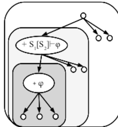
Figure 7: Assertion of \varphi
