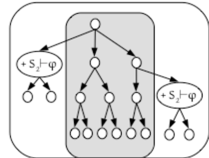
Figure 14: High negation of question
