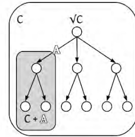
Figure 3: Update of commitment space C with speech act A; \sqrt{C} : root of C
