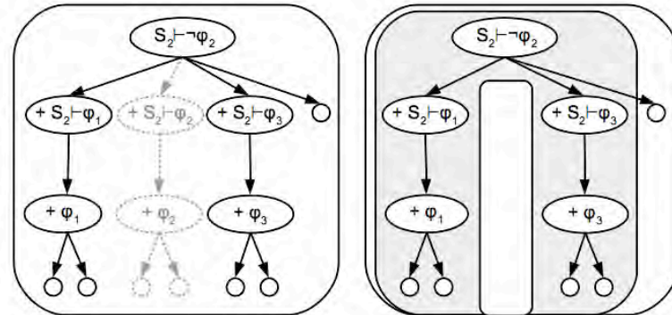
Figure 17: Remaining question after previous assertion of \neg \varphi_2
